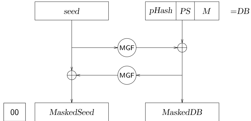
図 2.1: RSA-OAEP-Encode
